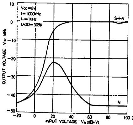
Fig. 28 AM detector output voltage vs. input voltage
